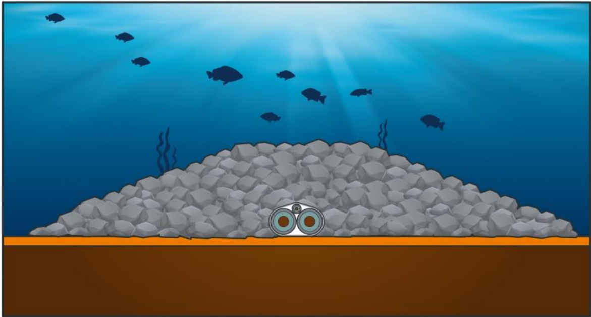
Figure 9 Schematic Cross-section of Rock Placement over the Submarine Cable
