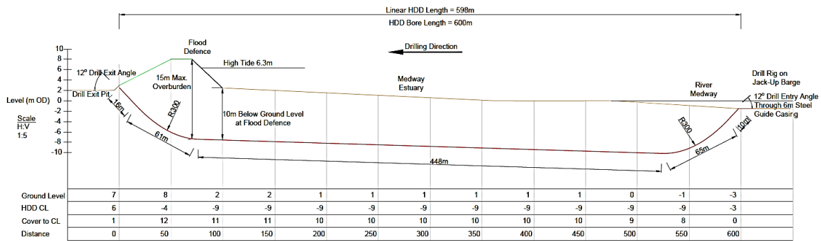
Figure 21 Schematic Cross-section of the Shore Crossing by Horizontal Directional Drilling at Kingsnorth
