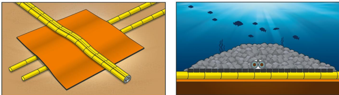
Figure 10 Schematic View of Placement of Concrete Mattresses at Crossing of Third Party Submarine Cable with Protection by Rock Placement
