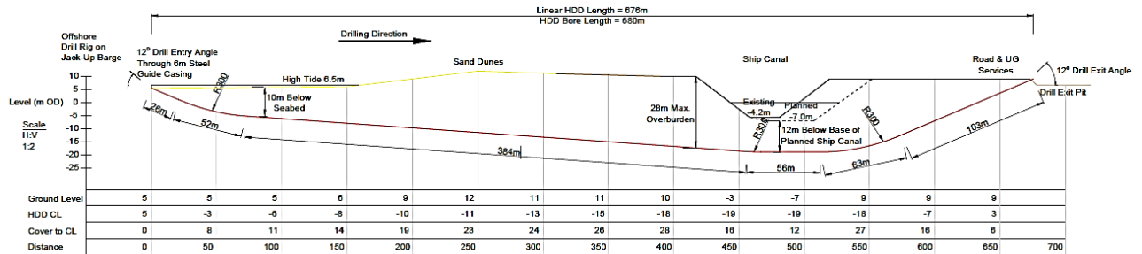
Figure 13 Schematic Cross-section of the Dunkerque Shore Crossing by Horizontal Directional Drilling (not to scale)
