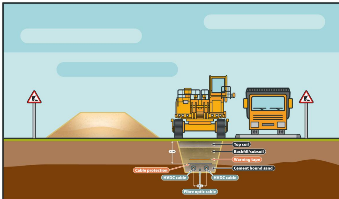
Figure 15 Schematic of the Cable Trench
