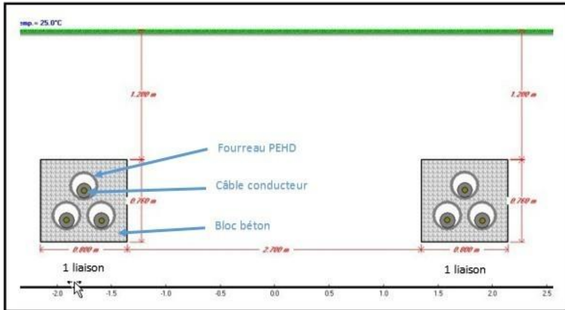
Figure 19 Schematic of Underground Double-circuit HVAC Cable Layout in Dunkerque (source: RTE)
