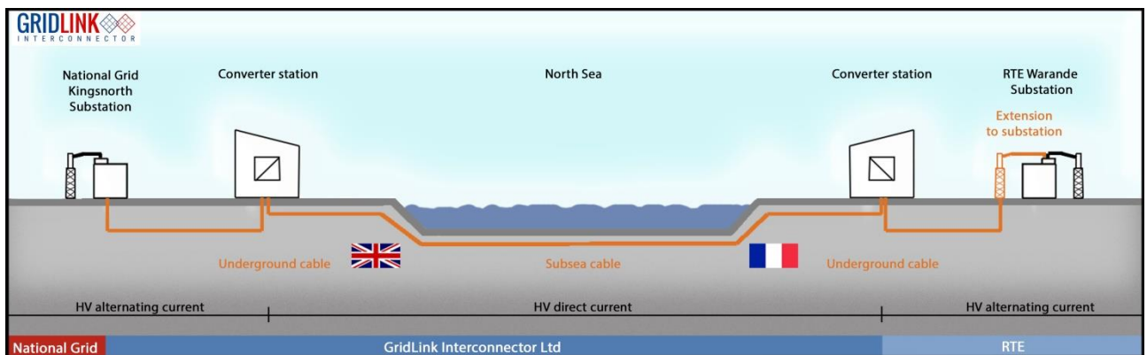
Figure 1 Schematic of the GridLink Project
