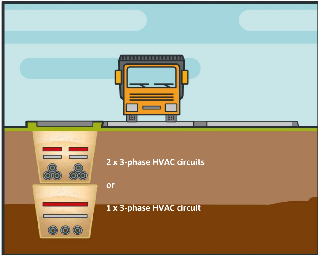
Figure 25 Schematic of Underground Cable Trench with One or Two HVAC Circuits in UK
